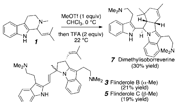
Scheme 4. Direct Methylative Dimerization
